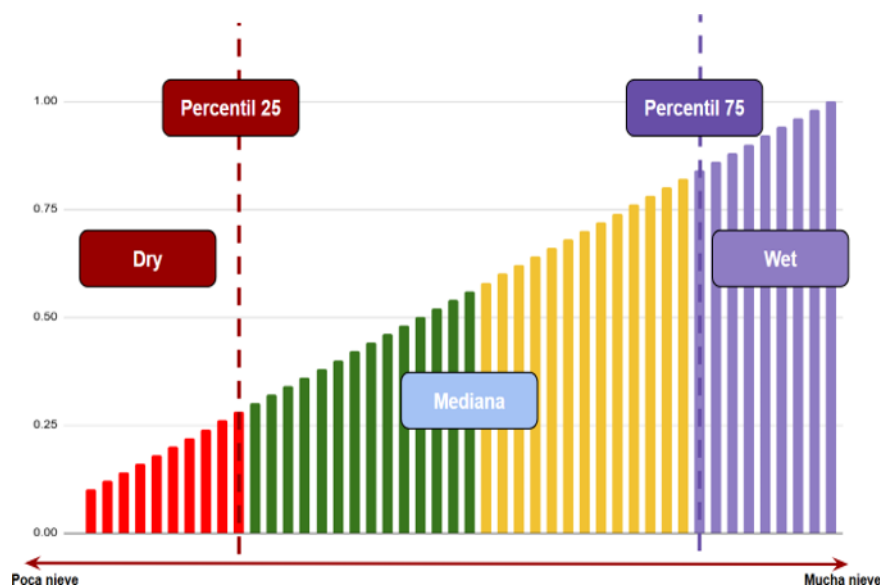
Figure 3: Construction of wet-season mosaics based on percentile distribution. Source: MapBiomias Peru.
