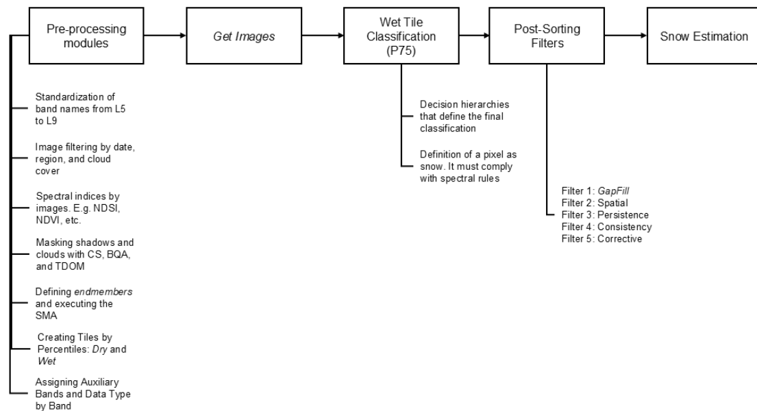
Figure 1. Methodological flowchart for the generation of snow-cover maps. Source: MapBiomass Peru.
