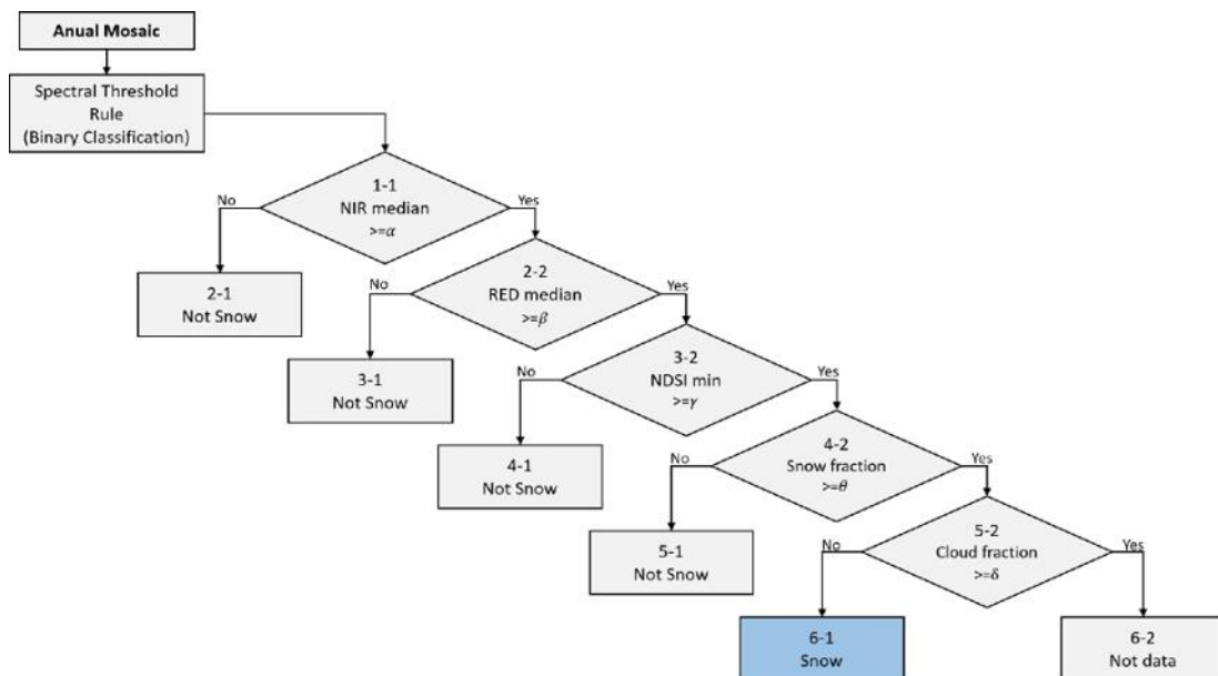
Figure 4: Empirical decision tree combined with Random Forest for snow classification. Source: MapBiomass Peru.
