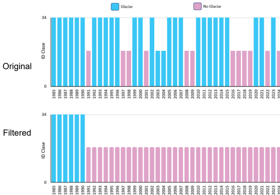
Figure 9: Temporal Persistence Filter
