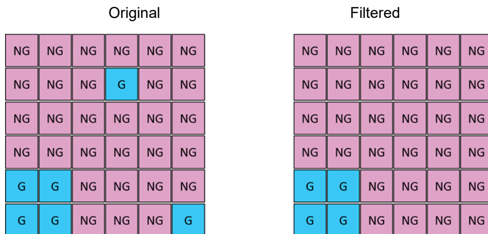
Figure 10: Spatial filter effect
