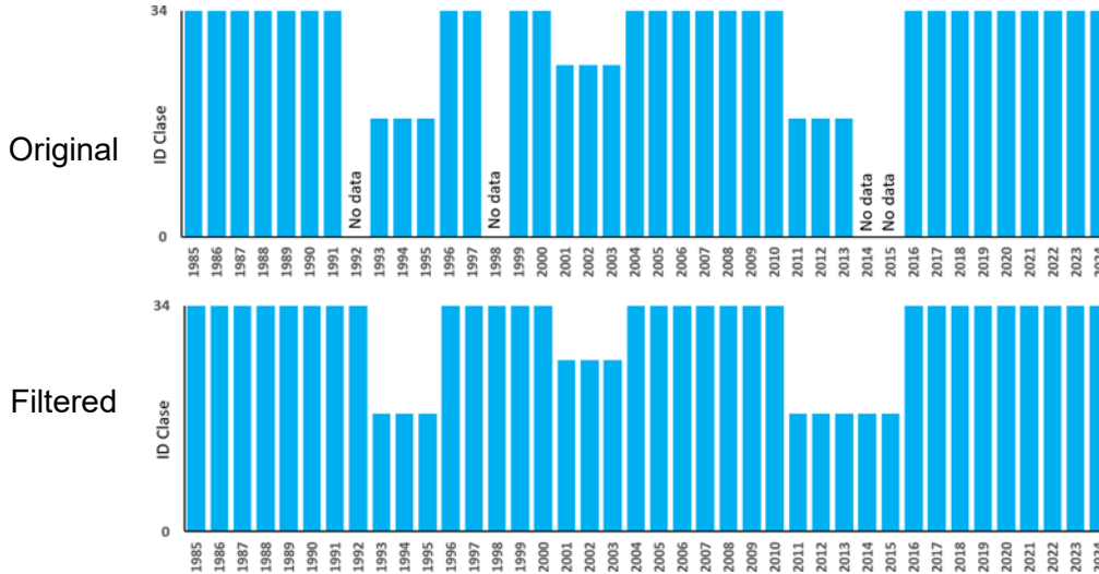
Figure 6: Gap Fill filter
