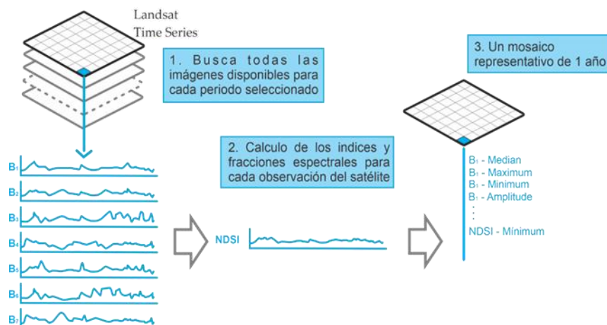
Figure 3: Creation of annual mosaics for Glaciers
