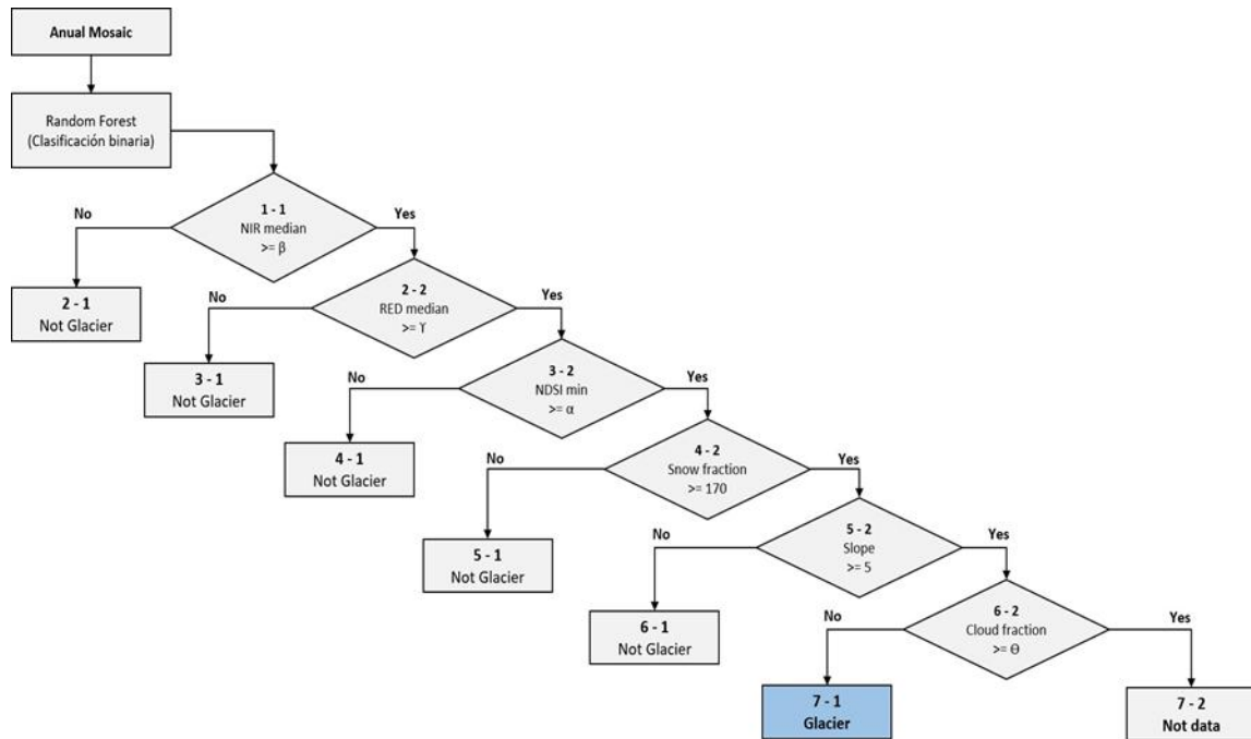
Figure 4: Empirical tree combined with Random Forest for glacier classification.
